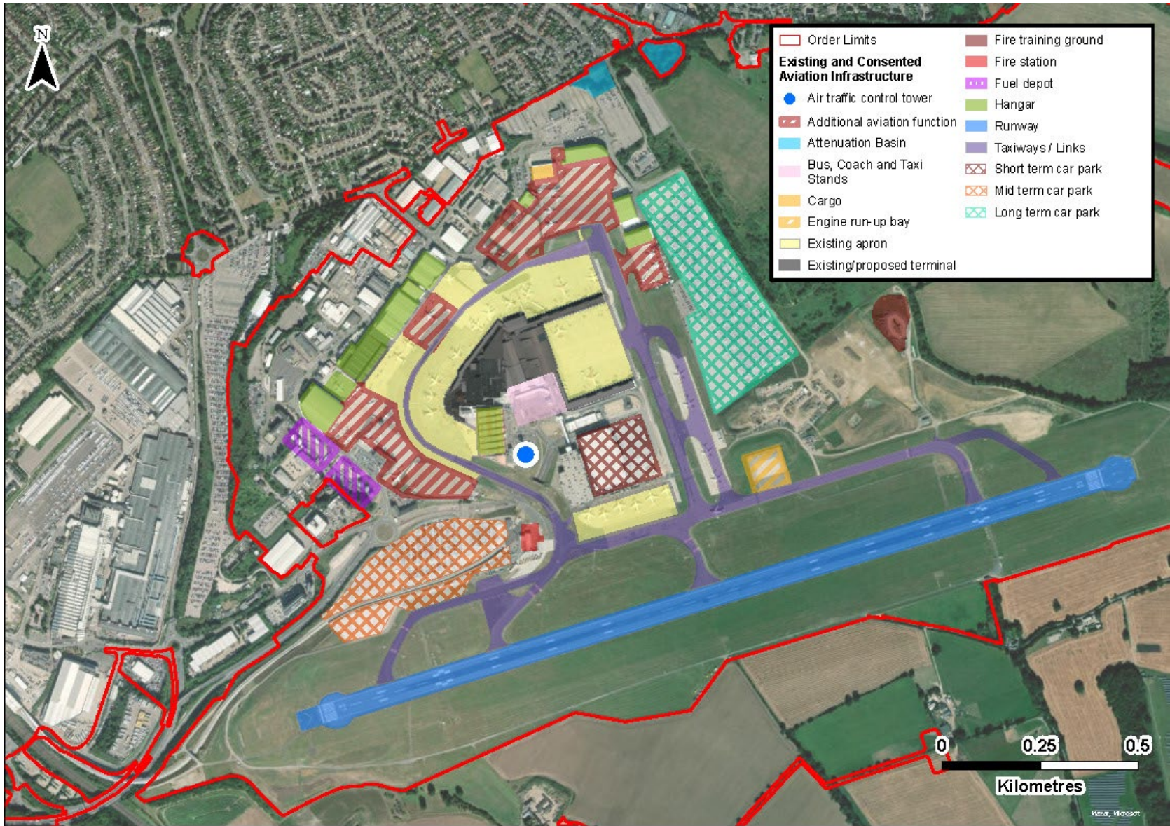
Figure 2.5: Existing Airport Layout
